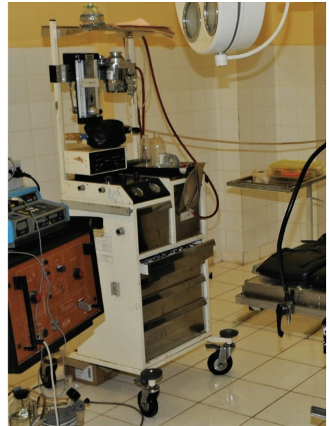
Figure 20. Modified, unsafe anaesthetic machine with no patient monitoring.
